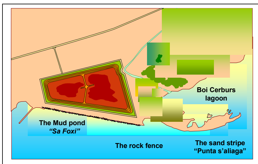
Figure 3.5: Location of TFM at the Sardinian refinery [33, Eurallumina, 2002]
