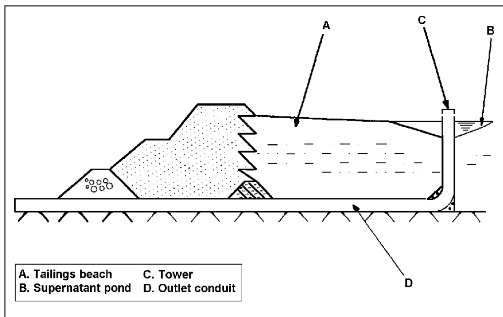
Figure 2.43: Tower decanting system [8, ICOLD, 1996]
